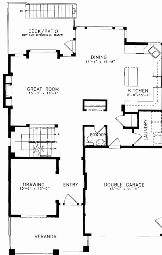
MAIN FLOOR PLAN: 1173 SQ. FT. GARAGE: 379 SQ. FT. VERANDA: 168 SQ. FT.
