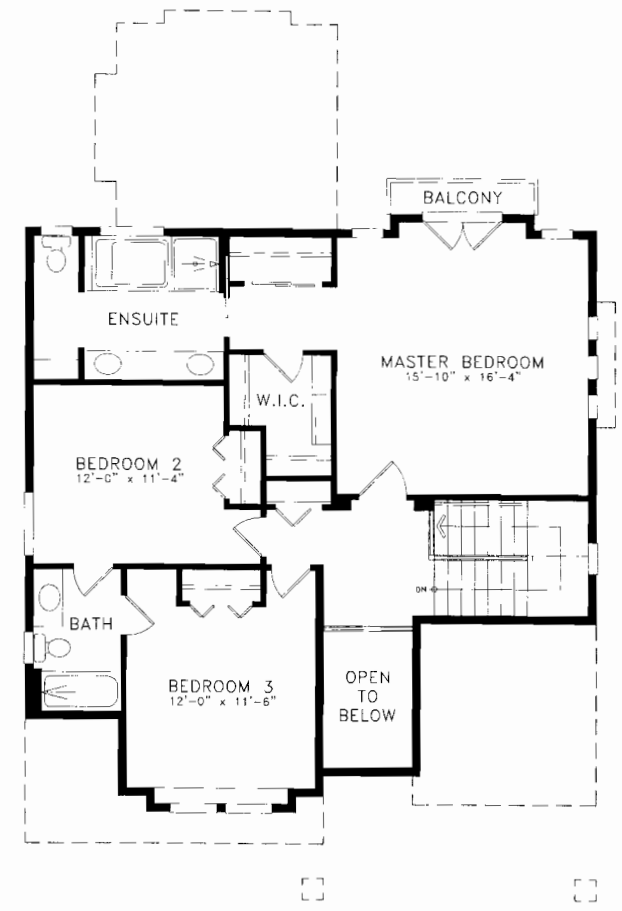
UPPER FLOOR PLAN: 1011 SQ. FT. BALCONY: 18 SQ. FT.
