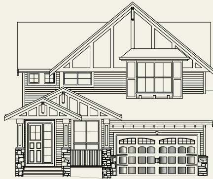
UPHILL ELEVATION B
