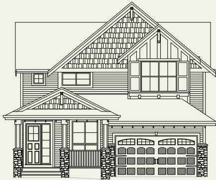
UPHILL ELEVATION A
