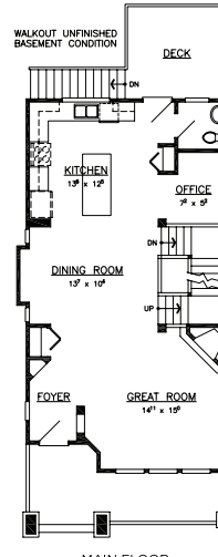
MAIN FLOOR 832 SQ. FT.
