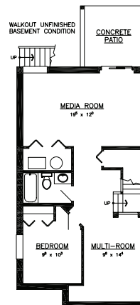
FINISHED BASEMENT 825 SQ. FT.
