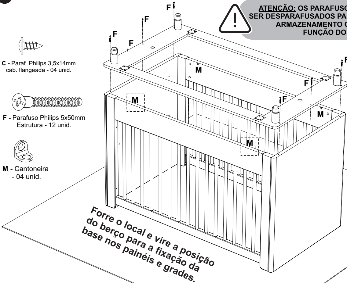
Trave as bases laterais nas barras da grade utilizando as cantoneiras (M) e parafusos (C).
