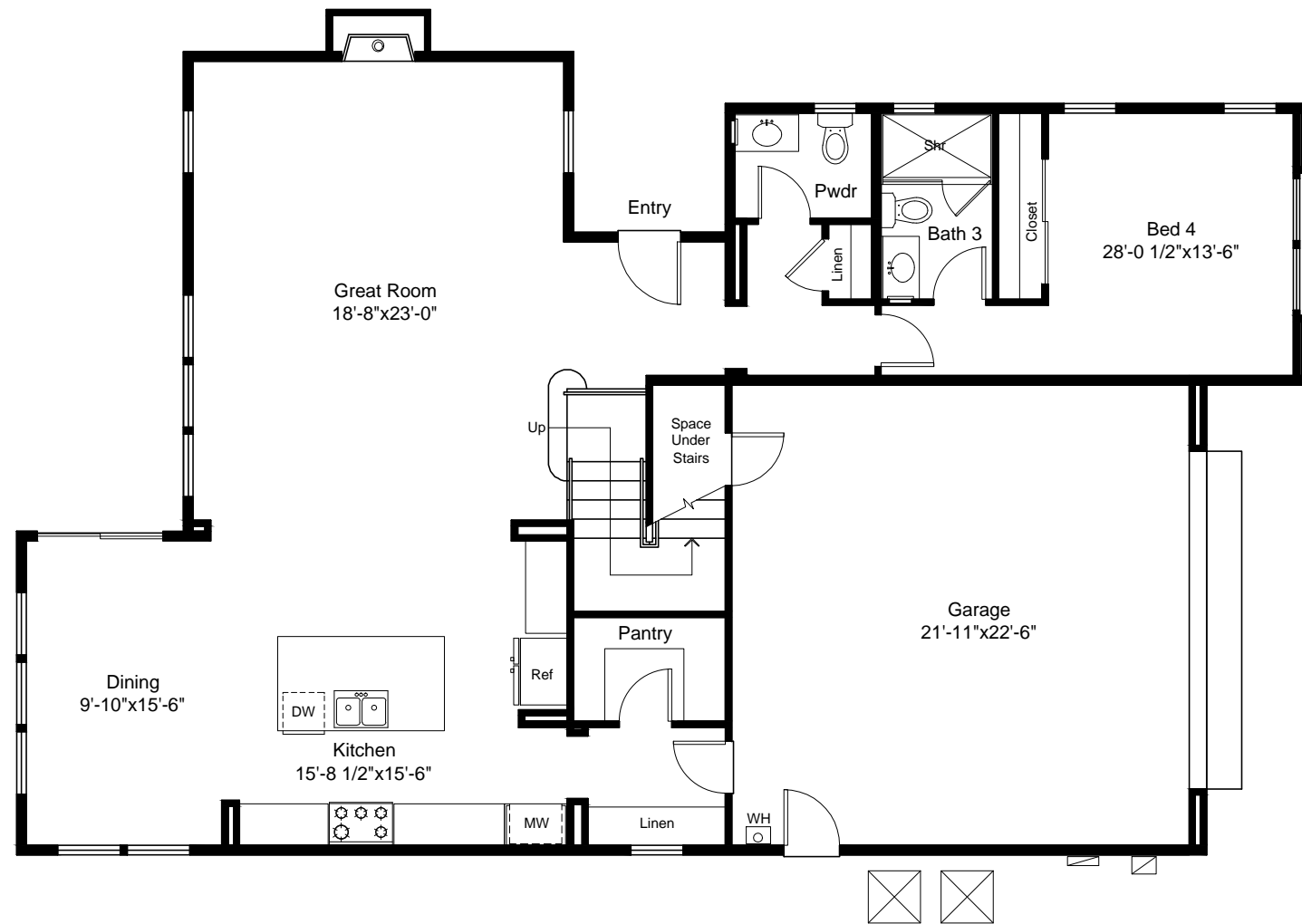
PLAN 1A FIRST FLOOR PLAN
