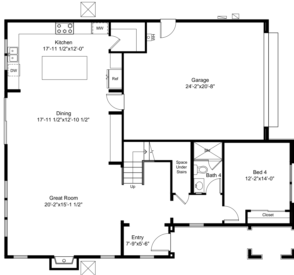
PLAN 2A-R FIRST FLOOR PLAN
