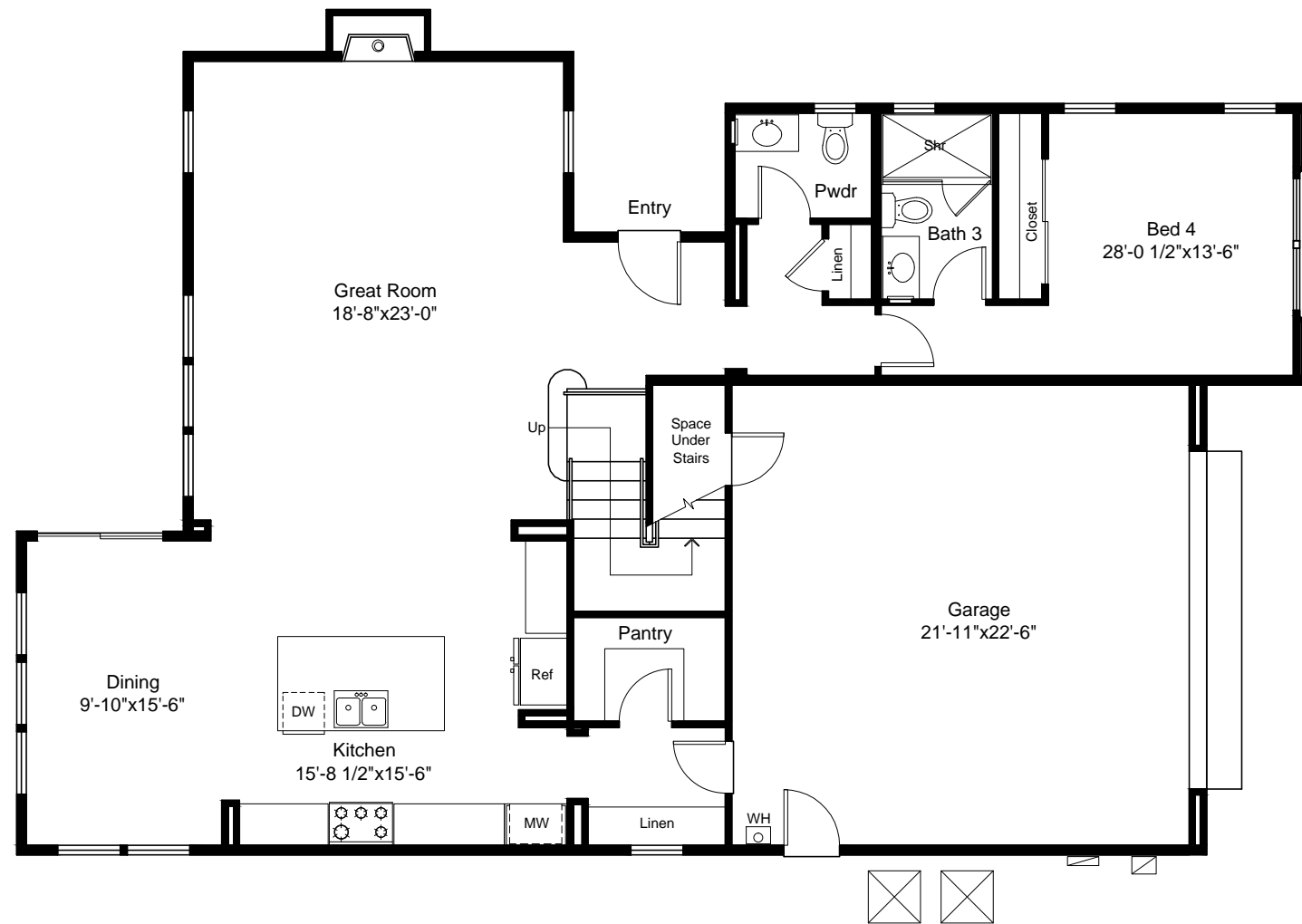
PLAN 1B FIRST FLOOR PLAN
