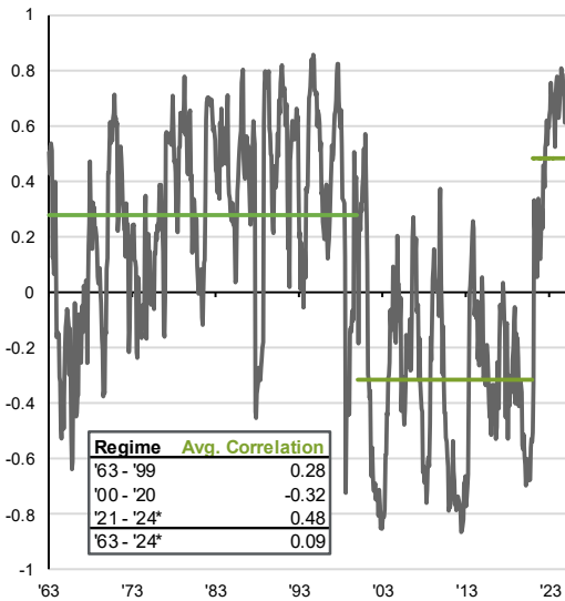
Rolling 12-month correlations S&P 500 and US 10-year Treasury
