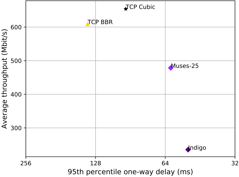
test from GCE Tokyo to GCE Sydney, 2 runs of 30s each per scheme (mean of all runs by scheme)
