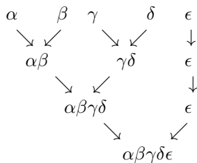
Figure 4: Example of closing a Merkle tree with an odd number of leaf nodes: the \epsilon node is promoted to its immediately upper level until it can be merged into the root.
