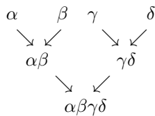
Figure 1: Example of Merkle tree with 4 hashes as leaf nodes.
