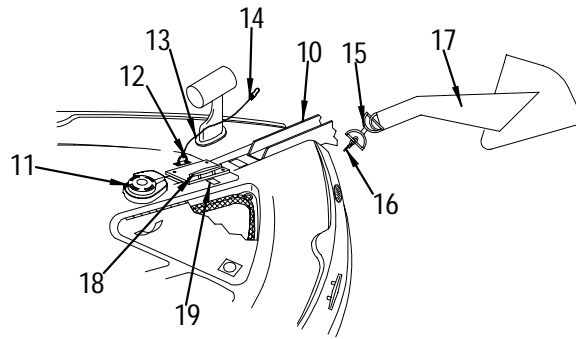
ANCHOR CHUTE W/ HAWSE PIPE OPTION
