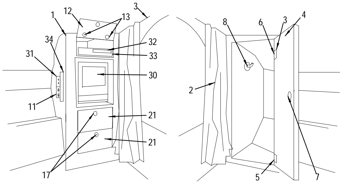
FORWARD STATEROOM STARBOARD
