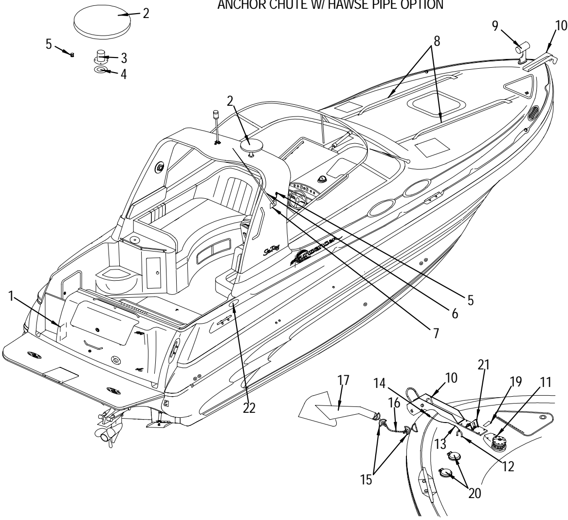
WINDLASS LOFRANS OPTION
