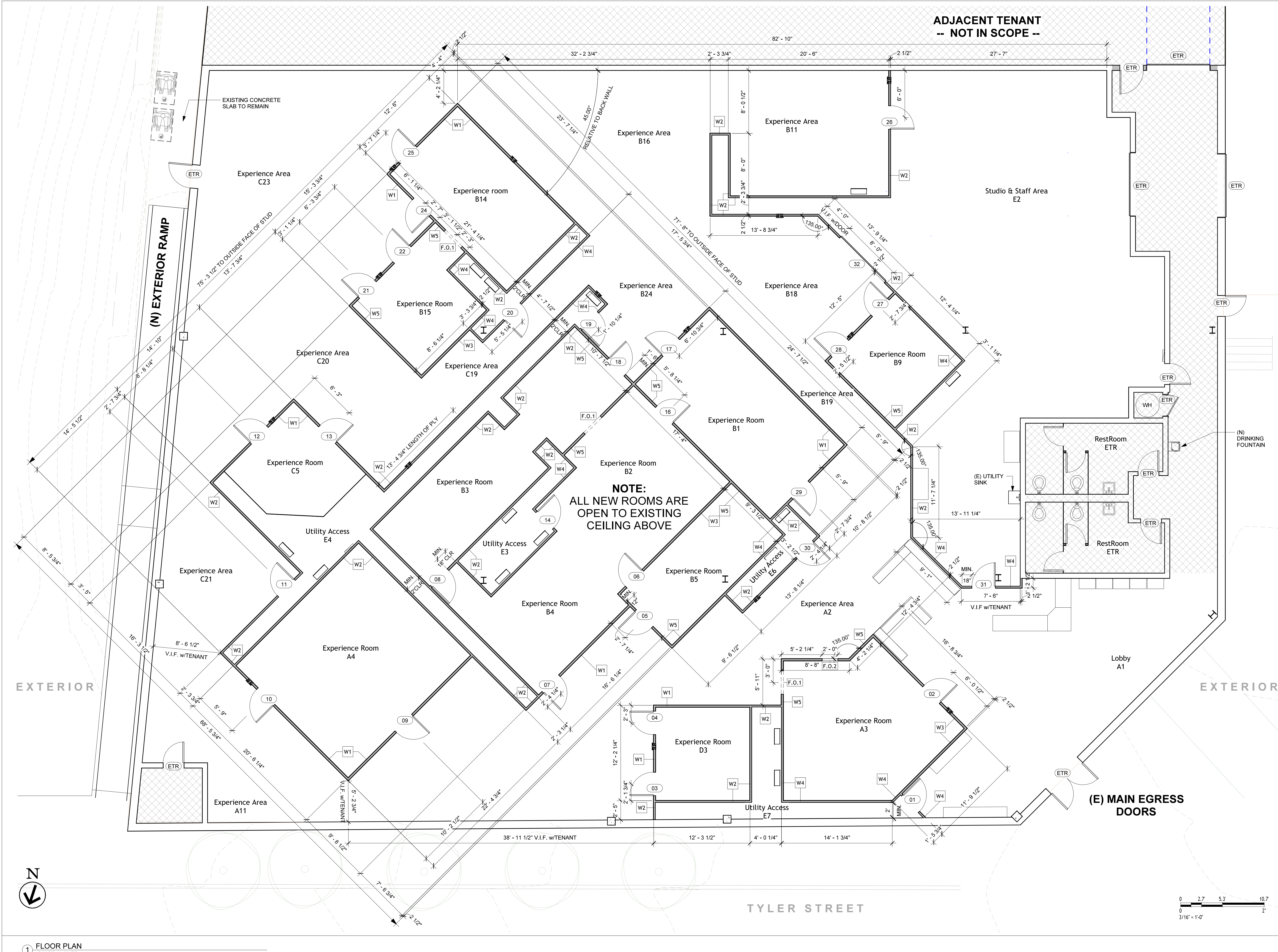
1 FLOOR PLAN 3/16" = 1'-0"
