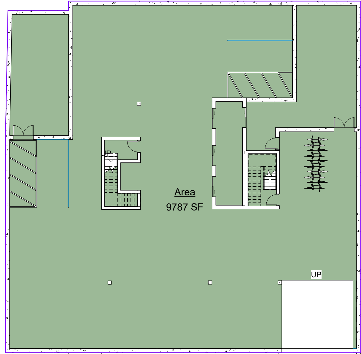
① 0 Garage Level 1/16" = 1'-0"
