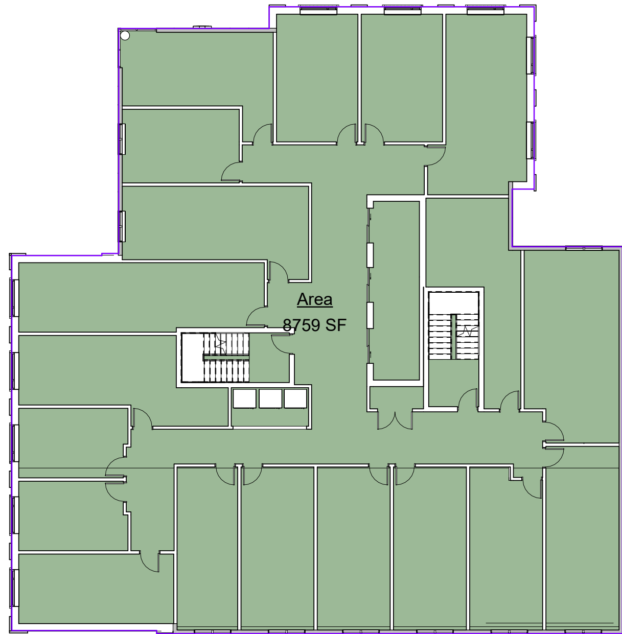
⑦ 6th Floor Level 1/16" = 1'-0"
