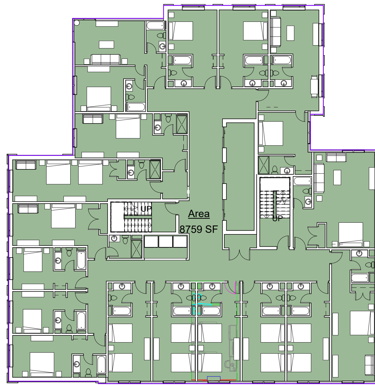
④ 3rd Floor Level 1/16" = 1'-0"
