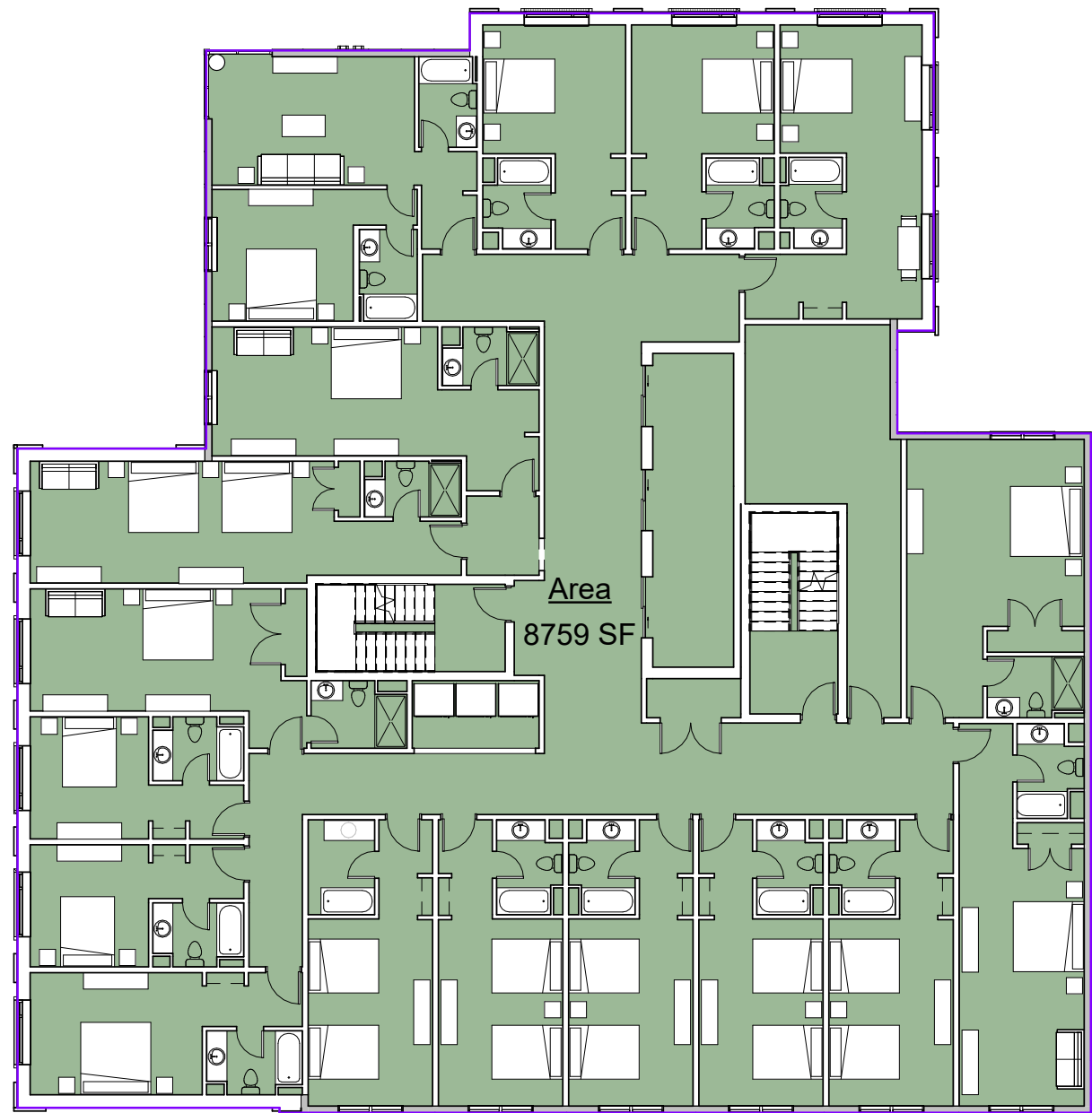
⑤ 4th Floor Level 1/16" = 1'-0"
