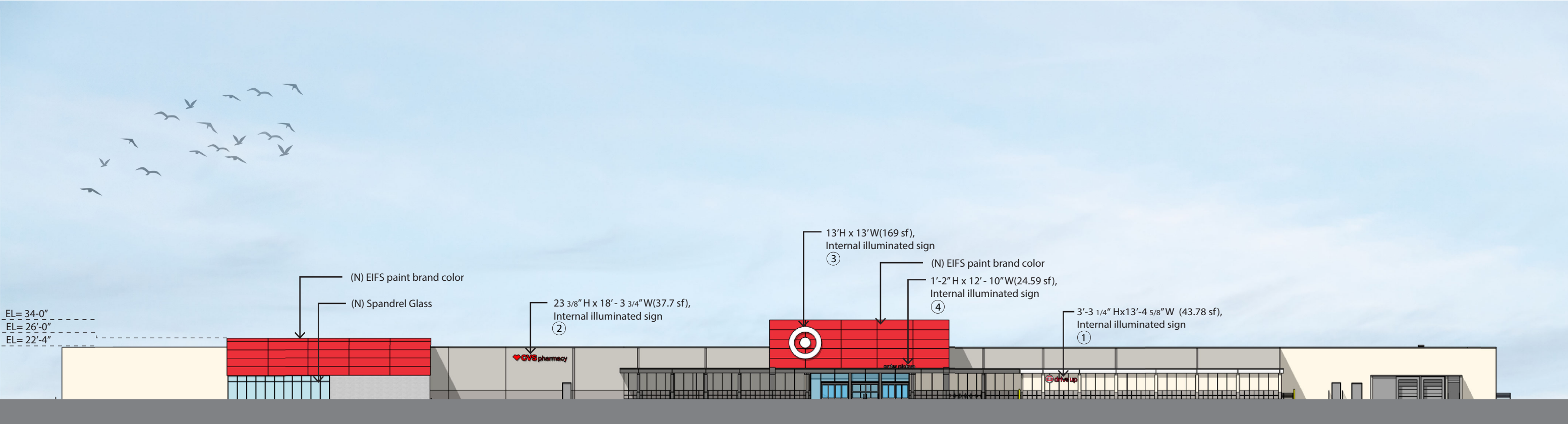
Front Elevation
