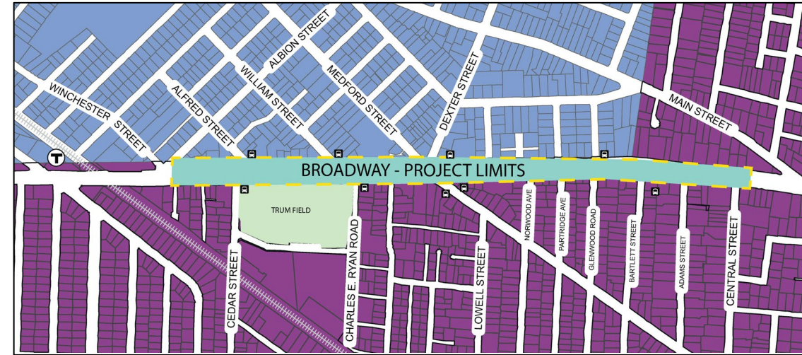
Extent of the Broadway Magoun Reconstruction Project
