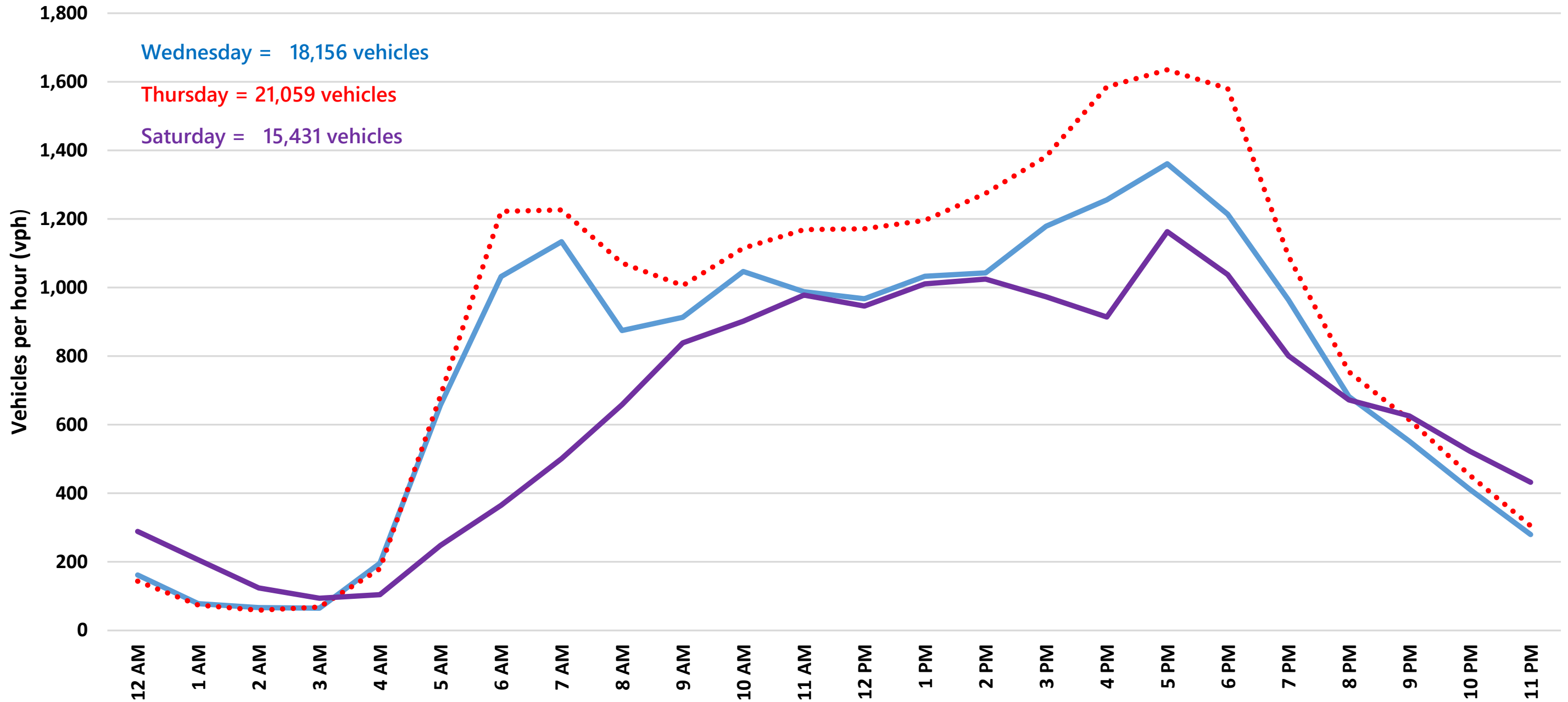
Figure 1 Mystic Avenue Observed Traffic Volumes
