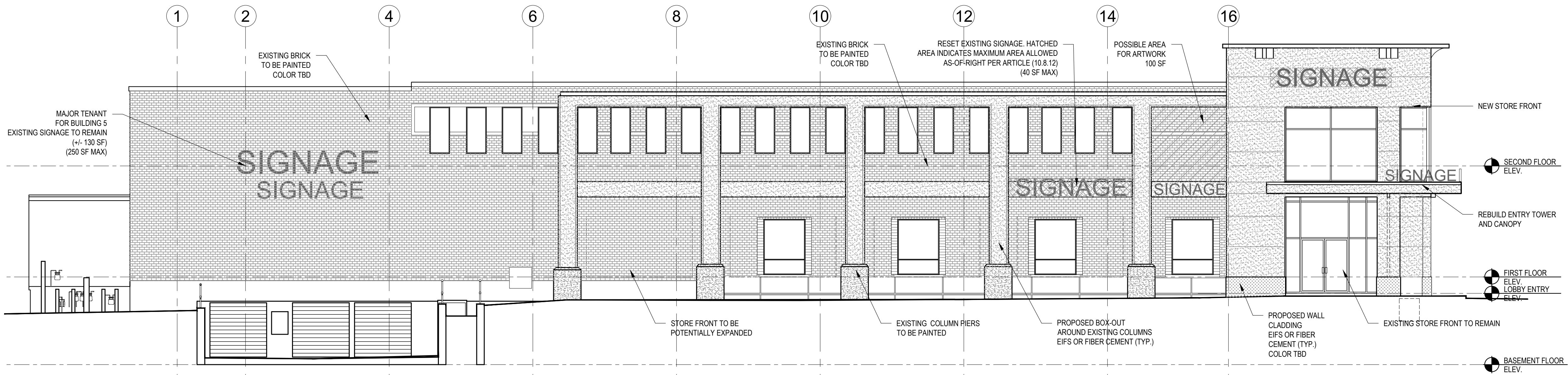
② BLDG 4- PROPOSED SIDE ELEVATION SCALE: 1/8"=1'-0"
