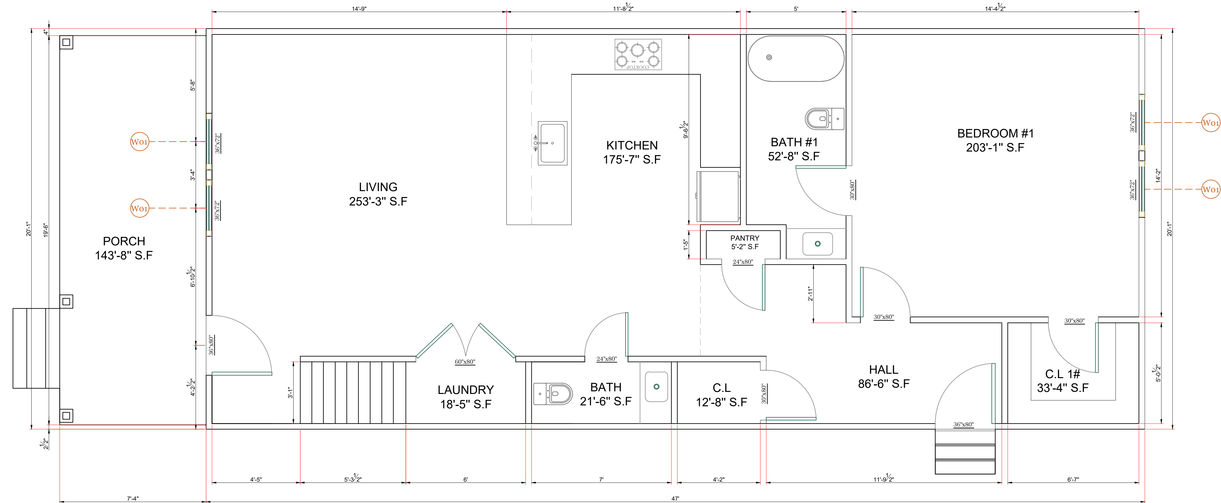
1 EXTERIOR DIMENSIONS PLAN SCALE: 3/4"
