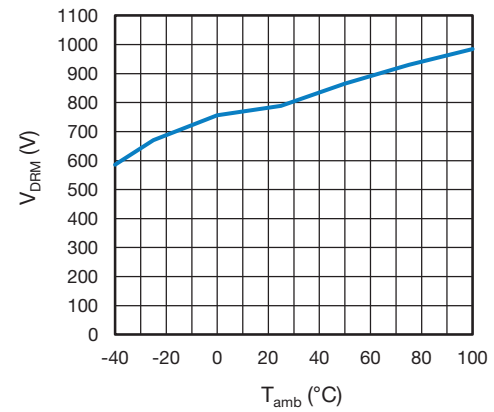
Fig. 14 - Peak Off-State Voltage vs. Ambient Temperature
