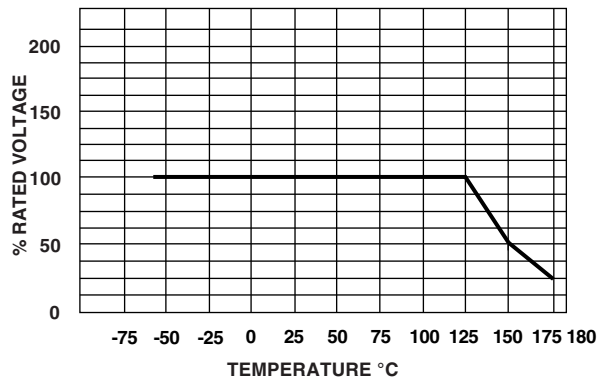
RATED VOLTAGE VS. TEMPERATURE
