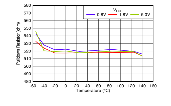
Figure 6-42. Smart Enable Pulldown Resistor vs Temperature and V_{OUT}
