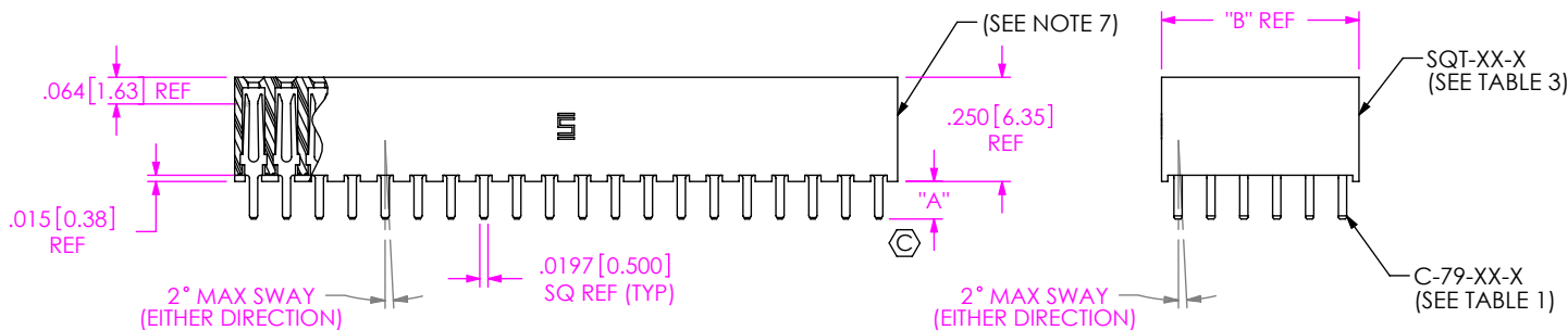
FIG 1 SQT-120-01-XX-6 SHOWN
