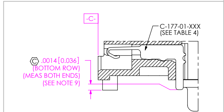
BOTTOM ROW - TAIL DETAIL (LOCATE ASSEMBLY ON DATUM -C- FOR MEASUREMENT)
