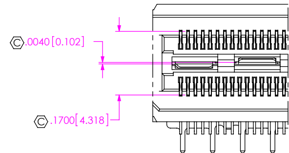
DETAIL 'D' SCALE 4 : 1
