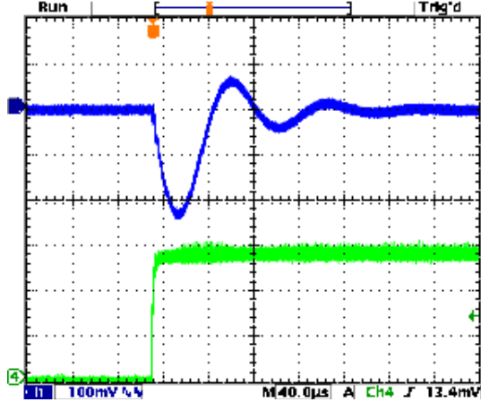
Step Load Transient Response (Vin=5.5V, Vout=3.3V, Load=10x10µF X5R 0805 ceramic, plus 1x470µF, 7mΩ POSCAP, total 570µF, Iout=0A to 1.5A) Top trace=Vout, Bottom trace=Iout
