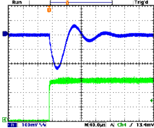
Step Load Transient Response (Vin=4.5V, Vout=1.8V, Clod=10x10µF X5R 0805 ceramic, plus 1x470µF, 7mΩ POSCAP, total 570µF, Iout=0A to 1.5A) Top trace=Vout, Bottom trace=Iout
