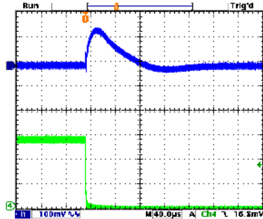
Step Load Transient Response (Vin=12V, Vout=3.3V, Load=10x10µF 5R 0805 ceramic, plus 1x470µF, 7mΩ POSCAP, total 570µF, Iout=1.5A to 0A) Top trace=Vout, Bottom trace=Iout
