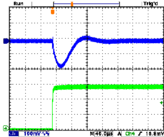
Step Load Transient Response (Vin=12V, Vout=3.3V, Load=10x10µF X5R 0805 ceramic, plus 1x470µF, 7mΩ POSCAP, total 570µF, Iout=0A to 1.5A) Top trace=Vout, Bottom trace=Iout
