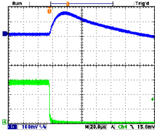
Step Load Transient Response (Vin=12V, Vout=1.8V, Clod=10x10µF X5R 0805 ceramic, plus 1x470µF, 7mΩ POSCAP, total 570µF, Iout=0A to 1.5A) Top trace=Vout, Bottom trace=Iout
