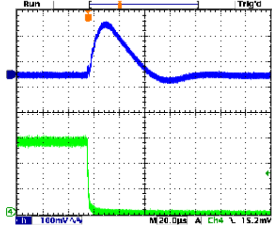
Step Load Transient Response (Vin=5.5V, Vout=3.3V, Load=10x10µF X5R 0805 ceramic, plus 1x470µF, 7mΩ POSCAP, total 570µF, Iout=1.5A to 0A) Top trace=Vout, Bottom trace=Iout
