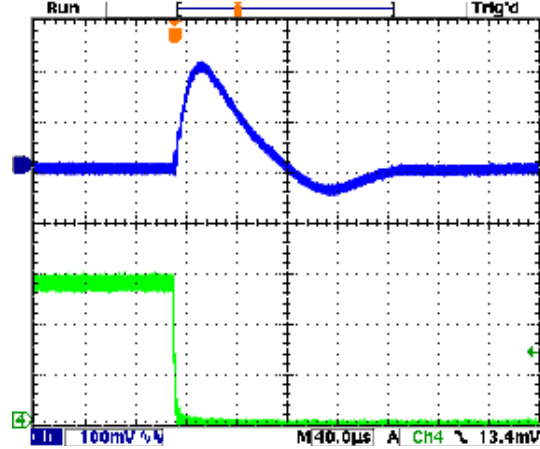
Step Load Transient Response (Vin=4.5V, Vout=1.8V, Clod=10x10µF X5R 0805 ceramic, plus 1x470µF, 7mΩ POSCAP, total 570µF, Iout=1.5A to 0A) Top trace=Vout, Bottom trace=Iout
