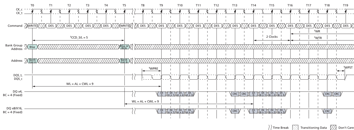
Figure 196: Consecutive WRITE (BC4-Fixed) with 1 st CK Preamble and Write CRC in Same or Different Bank Group
