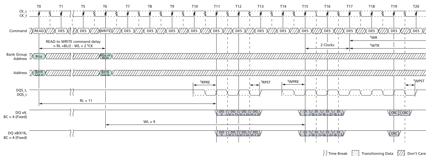
Figure 160: READ (BC4: Fixed) to WRITE (BC4: Fixed) with 1 st CK Preamble and Write CRC in Same or Different Bank Group
