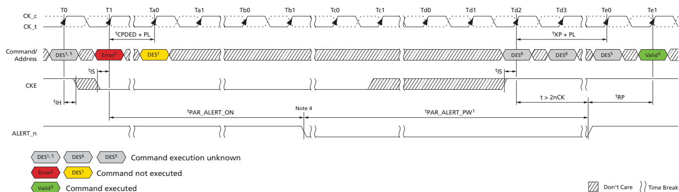
Figure 53: CA Parity Error Checking – SRE Attempt
