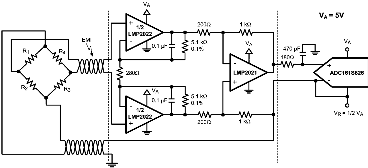
FIGURE 12. LMP2021/LMP2022 used with ADC161S626
