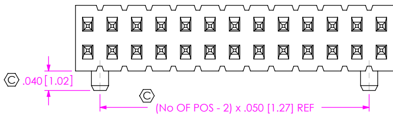
FIG 3 -A: ALIGNMENT PIN (STAKED) OPTION DIFFERENT AS SHOWN, OTHERWISE SAME AS FIG 2
