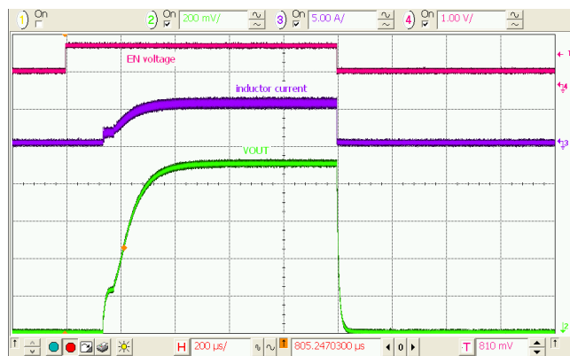
Figure 31. Startup / Shutdown, 180\text{ m}\Omega Load, V_{OUT} = 0.9\text{ V}
