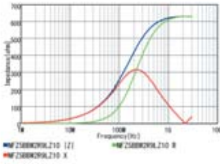
NFZ5BBW2R9LZ10
