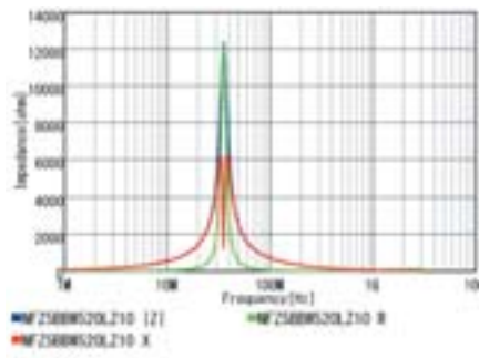
NFZ5BBW520LZ10
