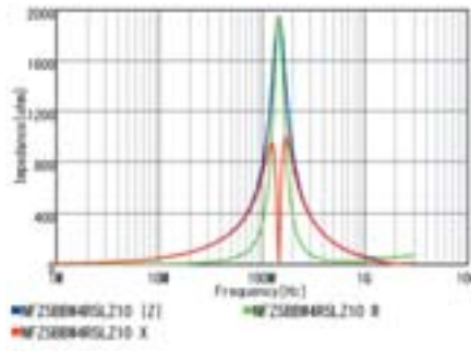
NFZ5BBW4R5LZ10
