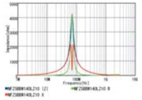
NFZ5BBW140LZ10
