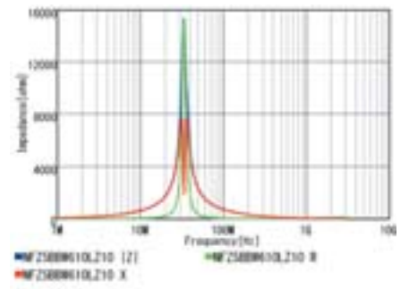
NFZ5BBW610LZ10
