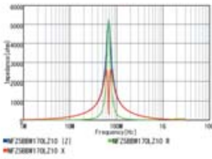
NFZ5BBW170LZ10
