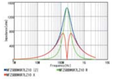
NFZ5BBW6R7LZ10
