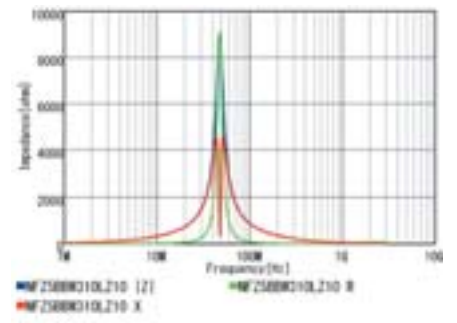
NFZ5BBW310LZ10
