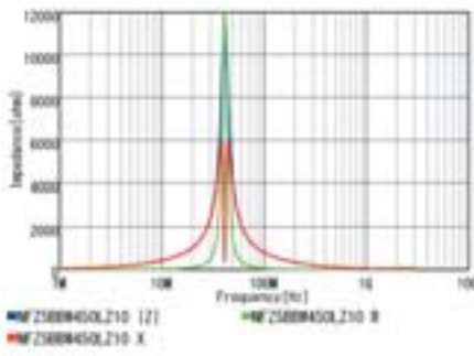
NFZ5BBW450LZ10
