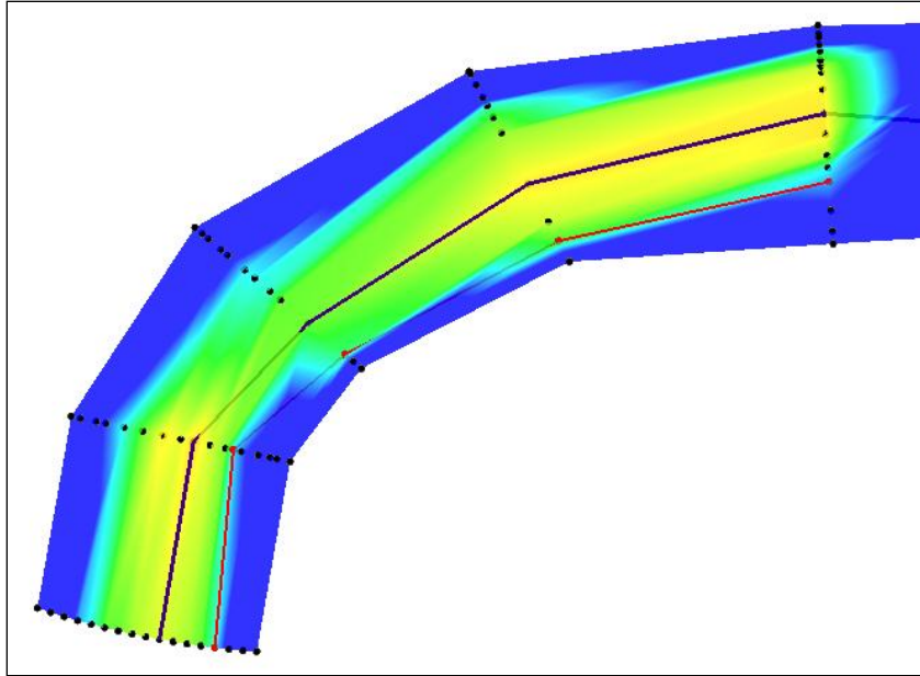
Figure 5 Creating the right bank toe
