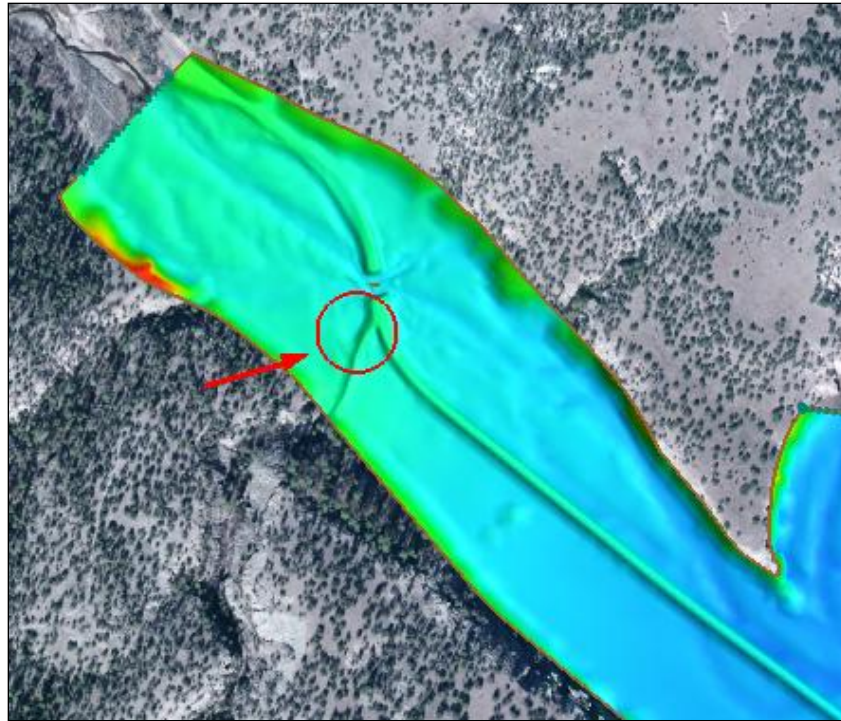
Figure 2 Weir location
