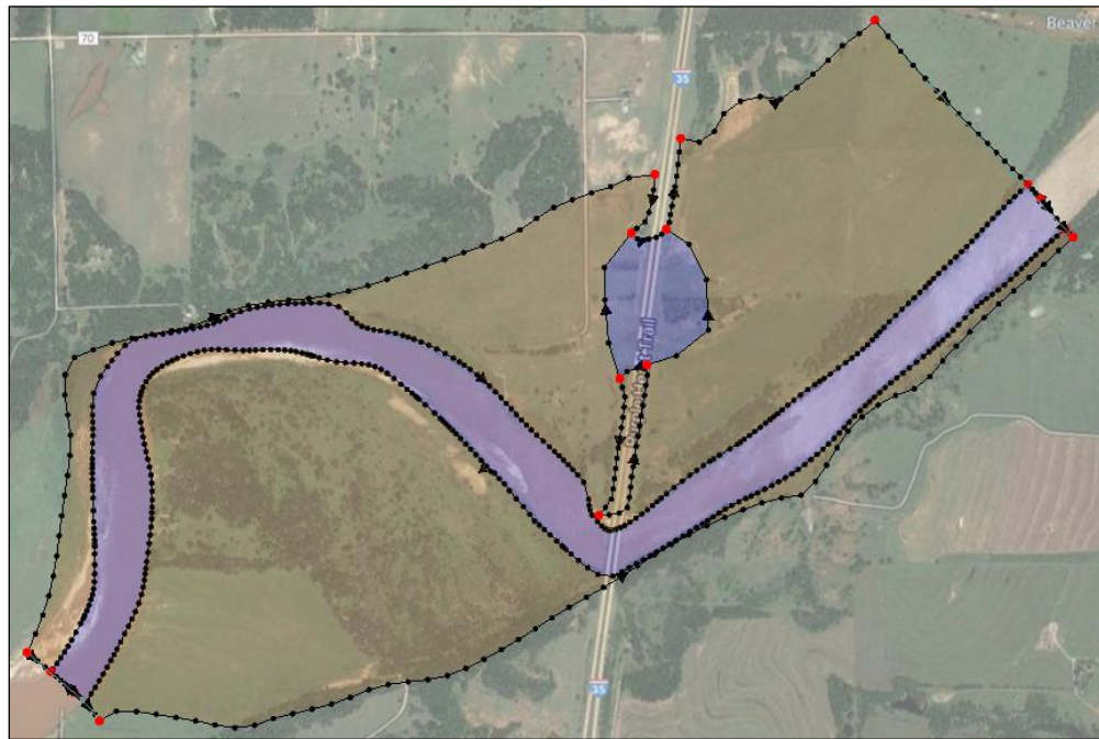
Figure 2 The two assigned material zones: the aqua color represents the channel areas, and the brown color represents the non-erodible areas
