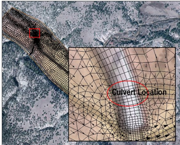
Figure 2 Culvert location
