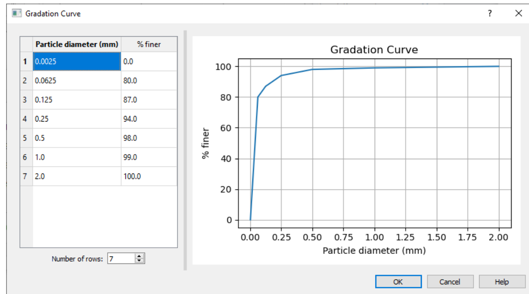
Figure 3 Sediment gradation curve for cohesive material
