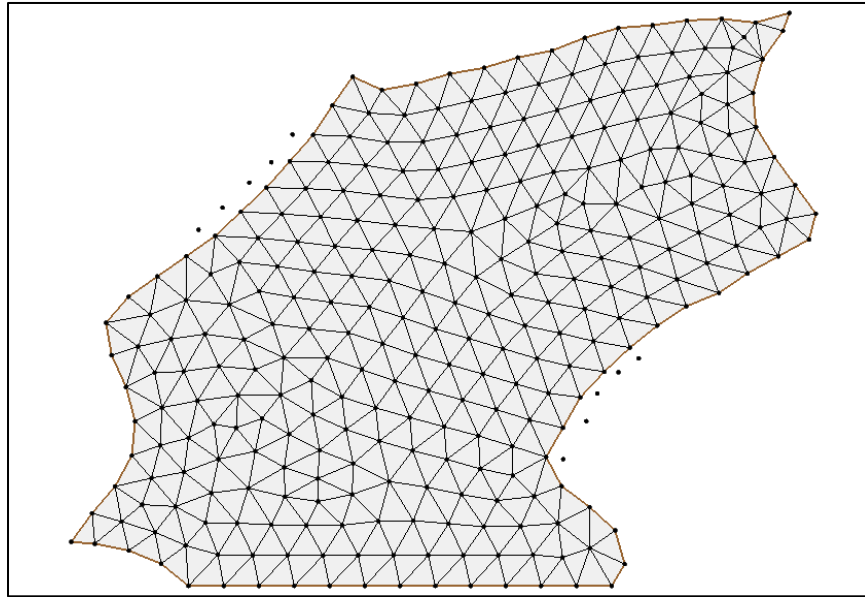
Figure 7 Merged UGrid
