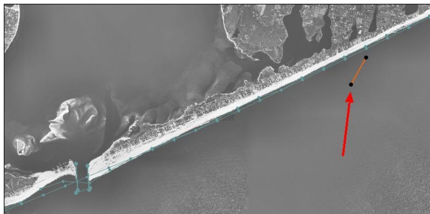
Figure 7 Breakwater northeast of Shinnecock Inlet
