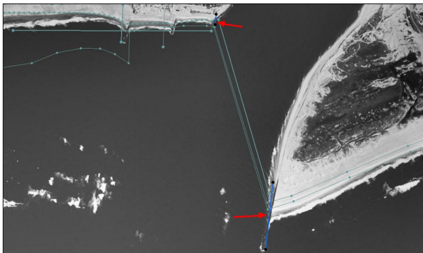
Figure 3 Jones Inlet with the two jetties indicated
