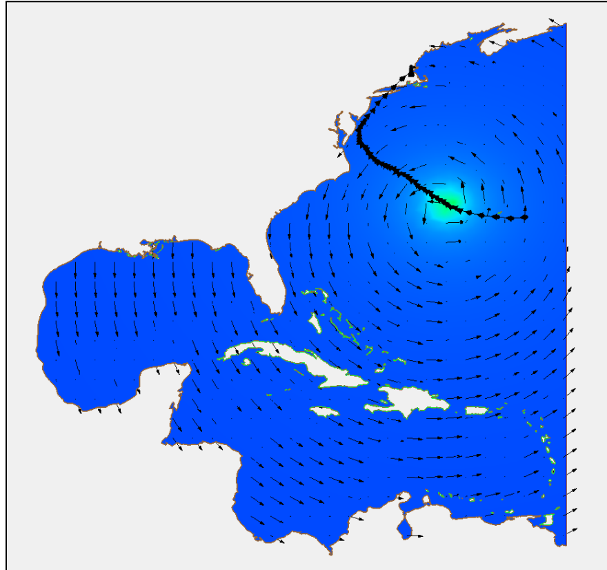
Figure 4 Symmetric cyclone visualization
