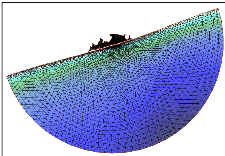
Figure 1 Initial mesh
