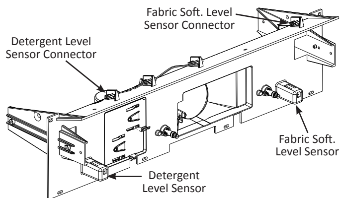
Figure 6 - Front of Metering Support Bracket
