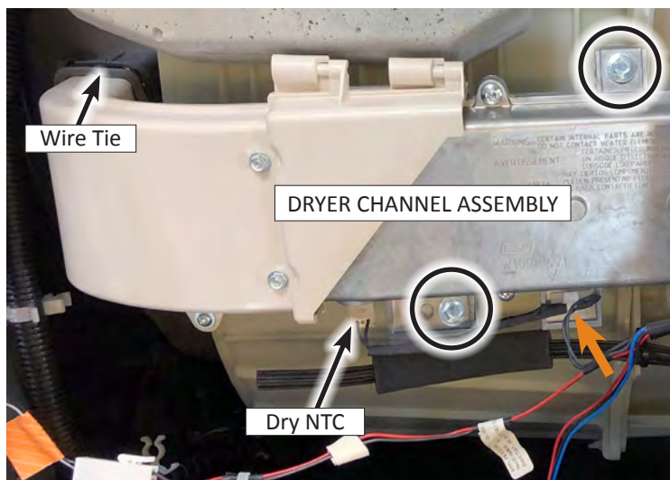
Figure 1 - Dryer Channel Assembly
