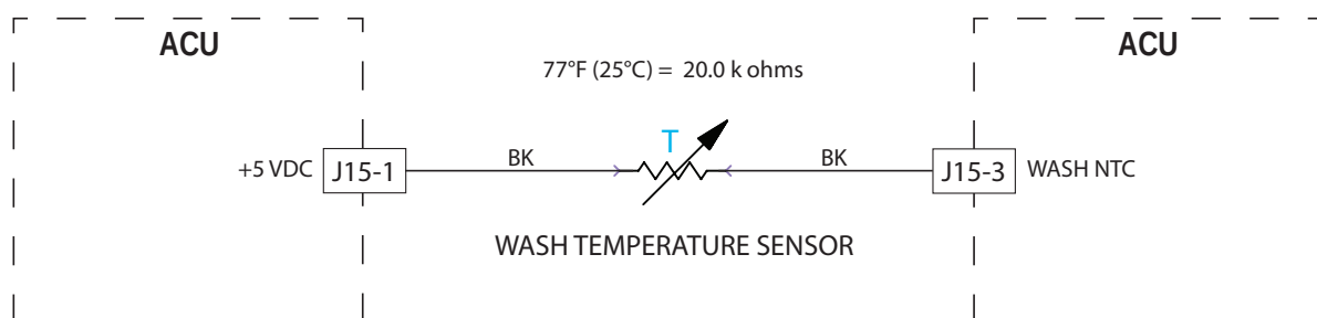
Figure 2 - Wash Temperature Sensor Strip Circuit
