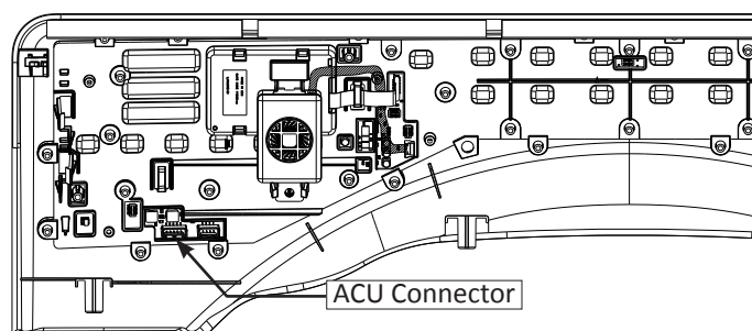
Figure 1 - Whirlpool Console HMI
