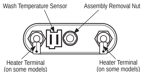
Figure 1 - Wash Temperature Sensor
