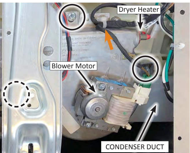
Figure 1 - Dryer Channel Assembly
