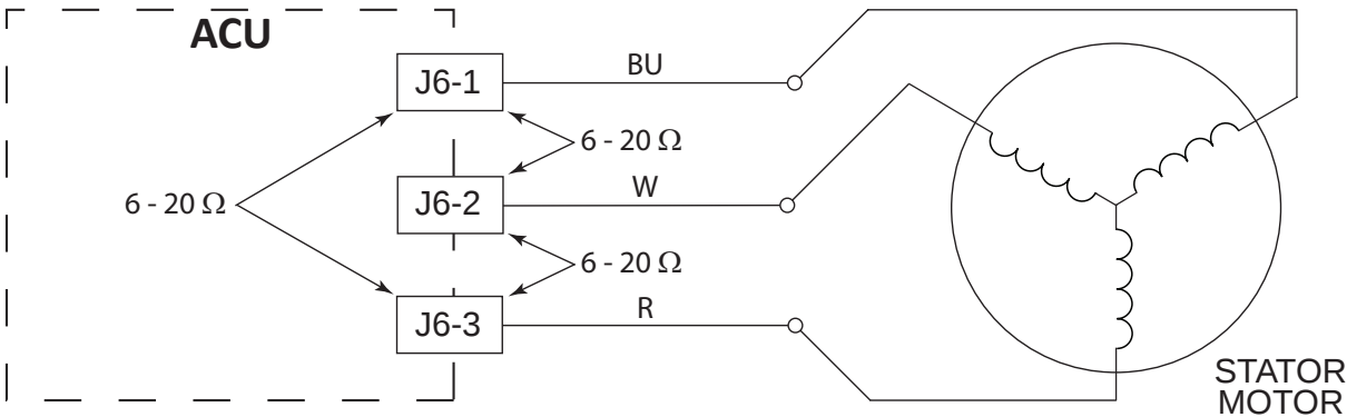
Figure 2 - Direct Drive Motor Strip Circuit
