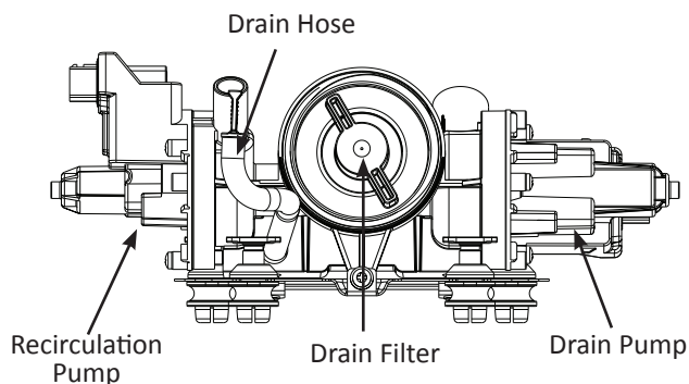
Figure 1 - Drain/Recirculation Pump
