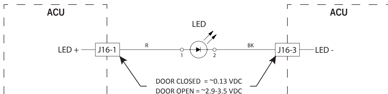
Figure 2 - Drum Light Strip Circuit
