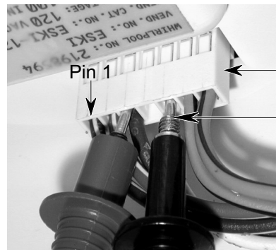
Test Leads
