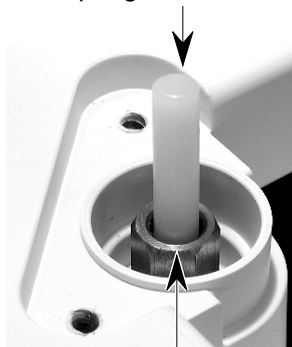
Top of Original Design Hex Drive Shaft
