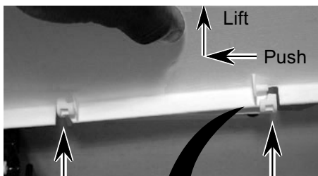
Ice Maker Door Pin
