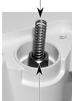
Top of Newly Designed Hex Drive Shaft
