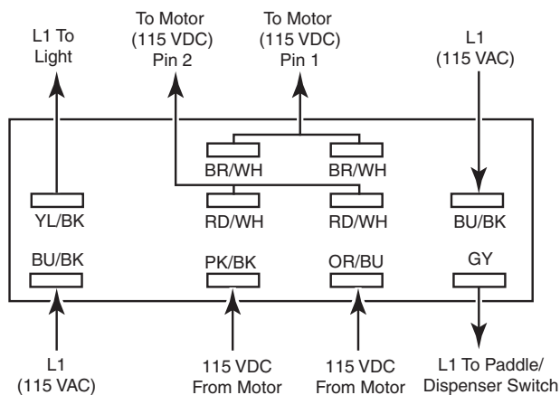
Switch Pack Pinouts
