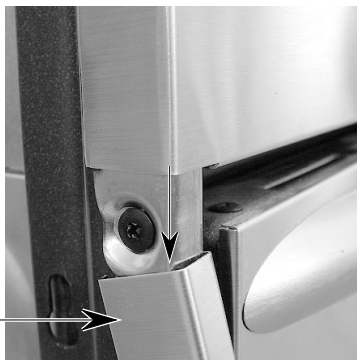
Pull Out Bottom Of Side Trim
