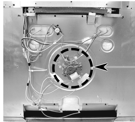
Convection Fan Motor Rear Screw (1 of 2)
