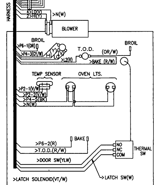
BACK VIEW LOWER OVEN
