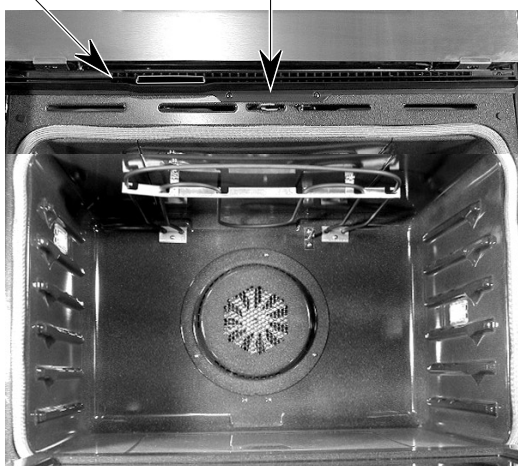
Lower Air Vent Lower Oven Door Latch Assembly
