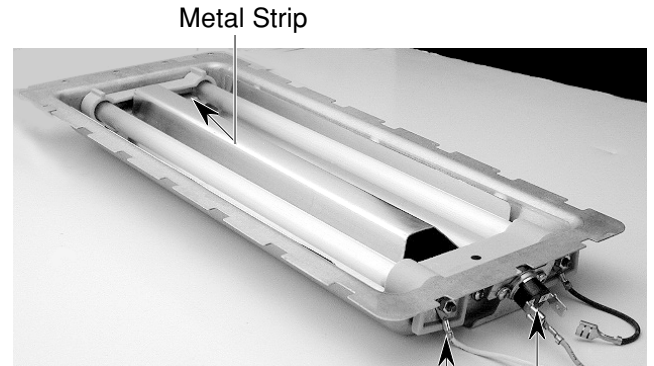
Metal Strip Element Screw Terminal (1 of 2) Grill Thermal Fuse
