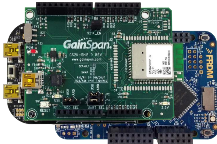
Wi-Fi Shield on NXP Freedom
