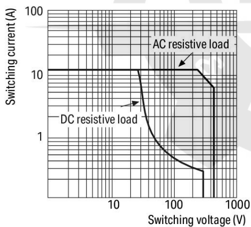
Load limit curve
