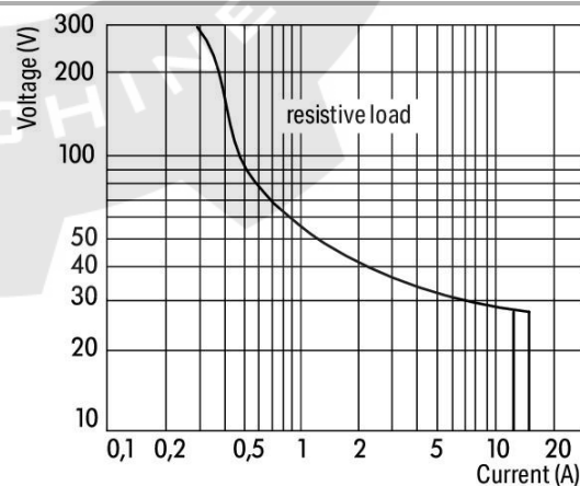
DC load limit curve
