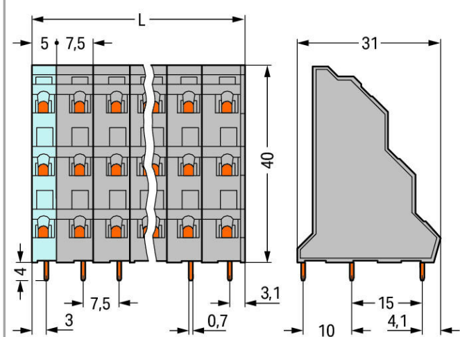
(1) Solder pins in a row
