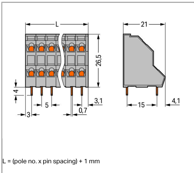
(1) Solder pins in a row
