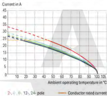
Derating Curve 1-conductor female connector (2231-102/026-000) with THT male header (231-162/001-000) Pin spacing: 5 mm / Conductor cross-section: 2.5 mm² *f-st* Based on: EN 60512-5-2 / Reduction factor: 0.8
