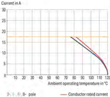
Current-Carrying Capacity Curve Pin spacing: 5 mm / Conductor cross-section: 1.5 mm² "f-st" Based on: EN 60512-5-2 / Reduction factor: 1
