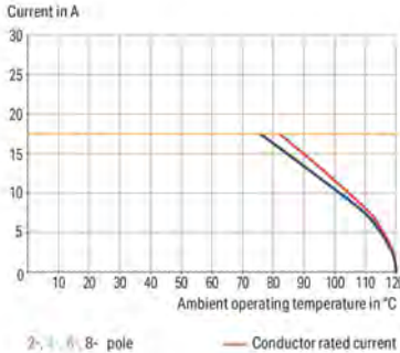
Current-Carrying Capacity Curve Pin spacing: 5 mm / Conductor cross-section: 1.5 mm² "f-st" Based on: EN 60512-5-2 / Reduction factor: 1
