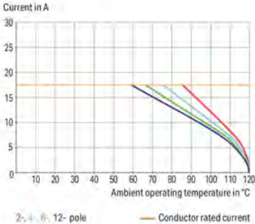
Current-Carrying Capacity Curve Pin spacing: 3.5 mm / Conductor cross-section: 1.5 mm² "f-st" Based on: EN 60512-5-2 / Reduction factor: 1
